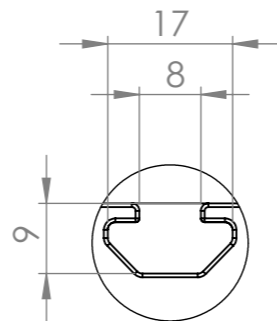
DETAIL A Type 30 T- slot SCALE 1 : 1
