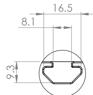
DETAIL A Type 30 T- slot SCALE 1 : 1
