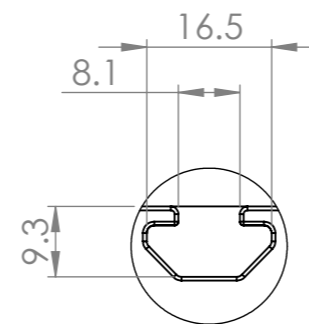
DETAIL A Type 30 T- slot SCALE 1 : 1
